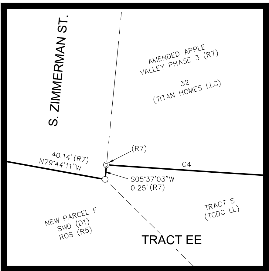
DETAIL A 1" = 1'
