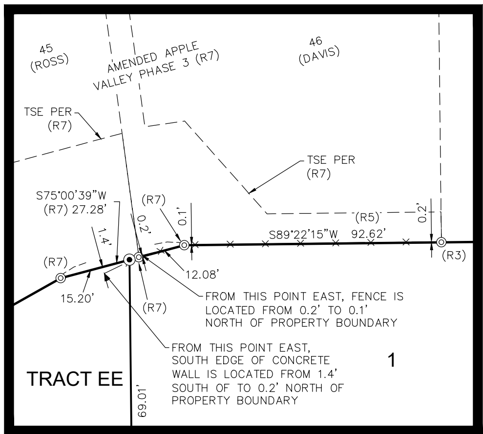
DETAIL B 1" = 20'
